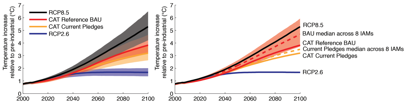
Figure 2.4: Projections for surface-air temperature increase
