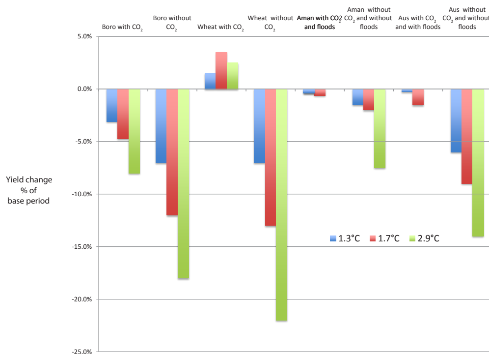
Figure 5.15: Median production change averaged across the climate change scenarios (A1B, A2, and B1) with and without CO 2 fertilization
