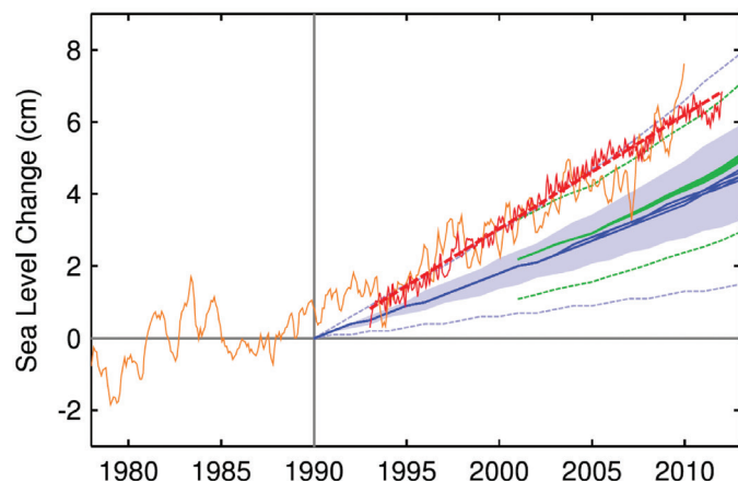
Figure 2.3: Sea-level rise from observations (orange: tide gauges, red: satellites) and models (blue: projections from IPCC TAR starting in 1990, green: projections from IPCC AR4 starting in 2000)
